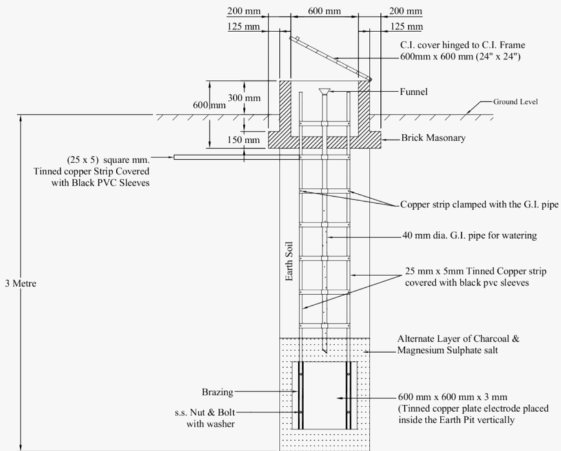
Fig: Method of Plate Earthing
