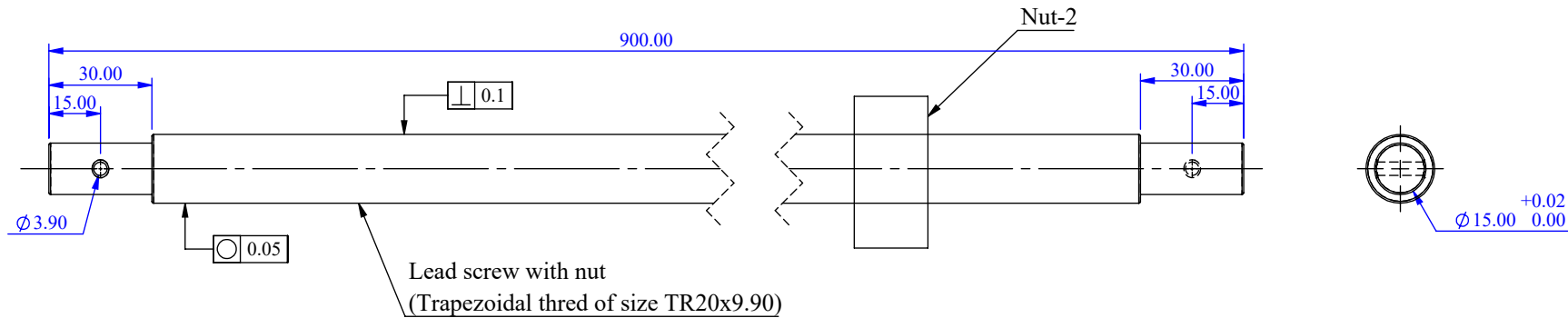
DETAILS OF LEAD SCREW-2 MATERIAL: SS-304 QTY.- 1 no.
